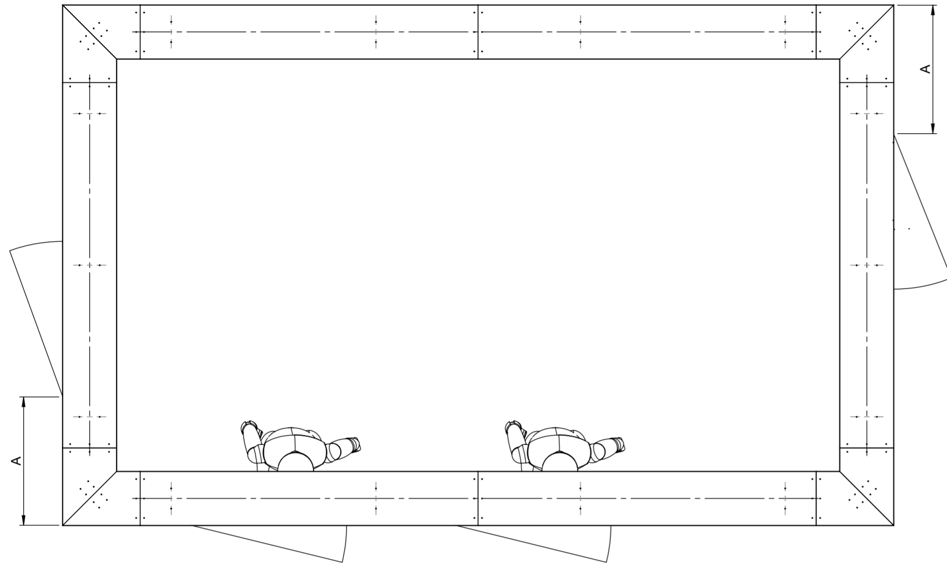
1 PLAN VIEW CLOSED CONCERTINA
